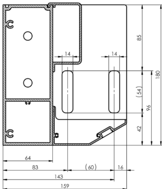
B3 - detail
